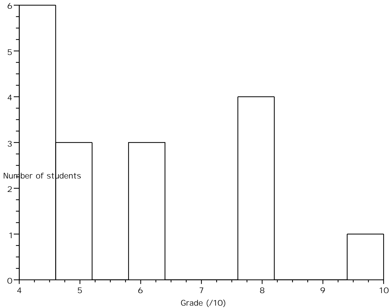
Histogram quiz 7
